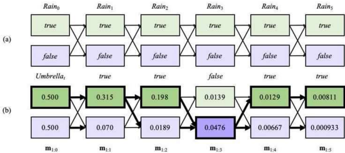
(a) Possible state sequences for Rain_t can be viewed as paths through a graph of the possible states at each time step. (States are shown as rectangles to avoid confusion with nodes in a Bayes net.) (b) Operation of the Viterbi algorithm for the umbrella observation sequence [true, true, false, true, true] , where the evidence starts at time 1. For each t , we have shown the values of the message m_{1:t} , which gives the probability of the best sequence reaching each state at time t . Also, for each state, the bold arrow leading into it indicates its best predecessor as measured by the product of the preceding sequence probability and the transition probability. Following the bold arrows back from the most likely state in m_{1:5} gives the most likely sequence, shown by the bold outlines and darker shading.
