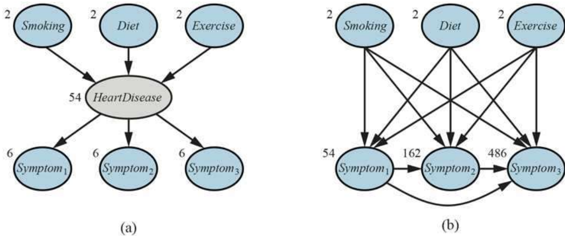
(a) A simple diagnostic network for heart disease, which is assumed to be a hidden variable. Each variable has three possible values and is labeled with the number of independent parameters in its conditional distribution; the total number is 78. (b) The equivalent network with HeartDisease removed. Note that the symptom variables are no longer conditionally independent given their parents. This network requires 708 parameters.
