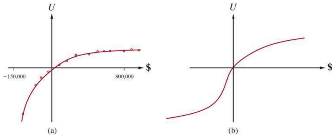
The utility of money. (a) Empirical data for Mr. Beard over a limited range. (b) A typical curve for the full range.
