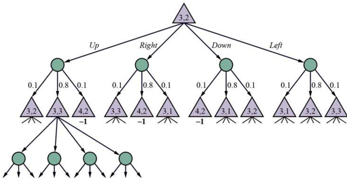
Part of an expectimax tree for the 4 \times 3 MDP rooted at (3,2) . The triangular nodes are max modes and the circular nodes are chance nodes.
