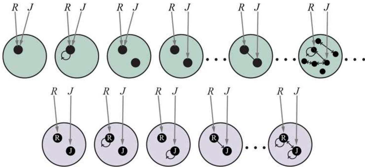
Top: Some members of the set of all possible worlds for a language with two constant symbols, R and J , and one binary relation symbol, under the standard semantics for first-order logic. Bottom: the possible worlds under database semantics. The interpretation of the constant symbols is fixed, and there is a distinct object for each constant symbol.
