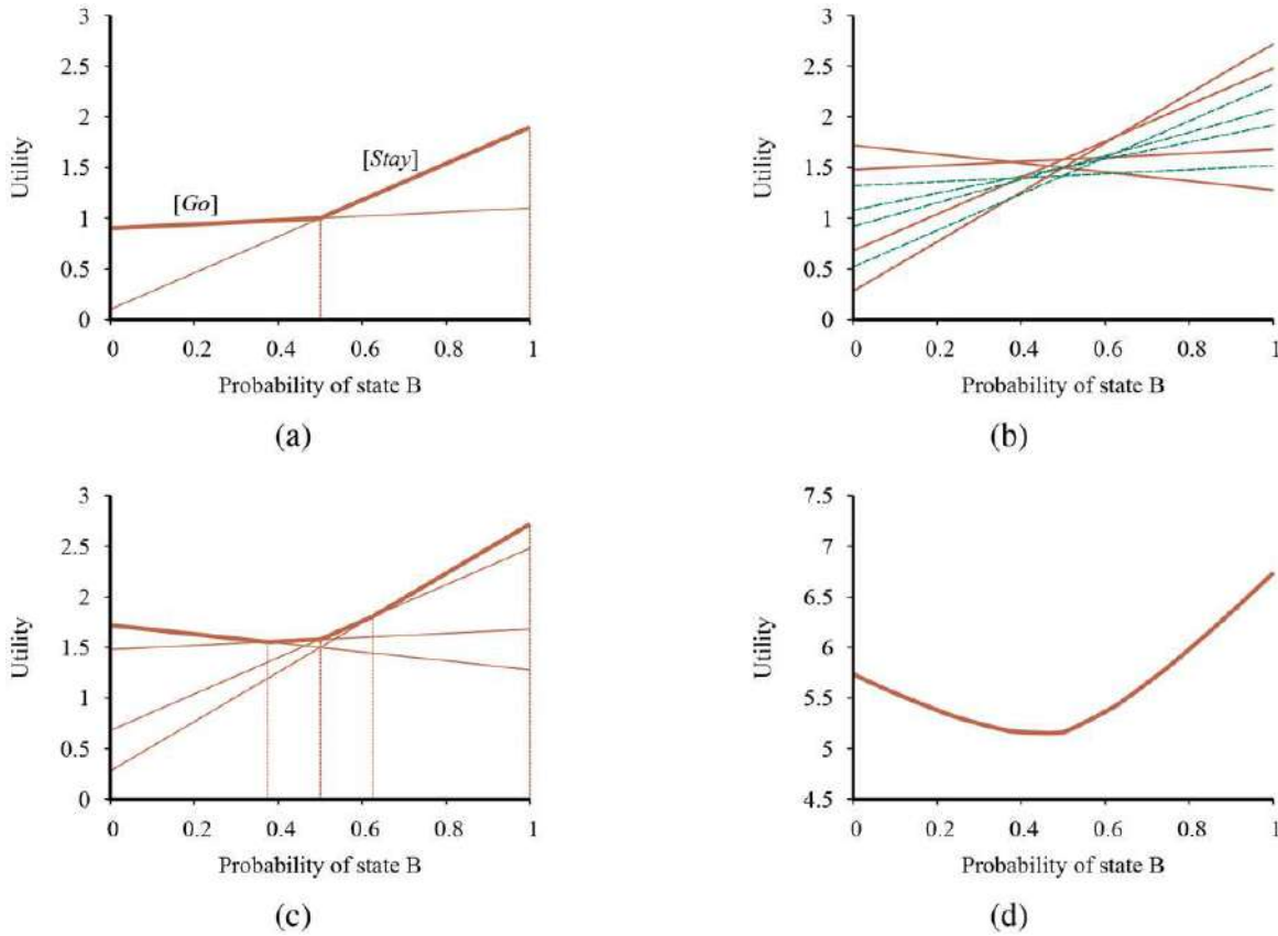
(a) Utility of two one-step plans as a function of the initial belief state b(B) for the two-state world, with the corresponding utility function shown in bold. (b) Utilities for 8 distinct two-step plans. (c) Utilities for four undominated two-step plans. (d) Utility function for optimal eight-step plans.
