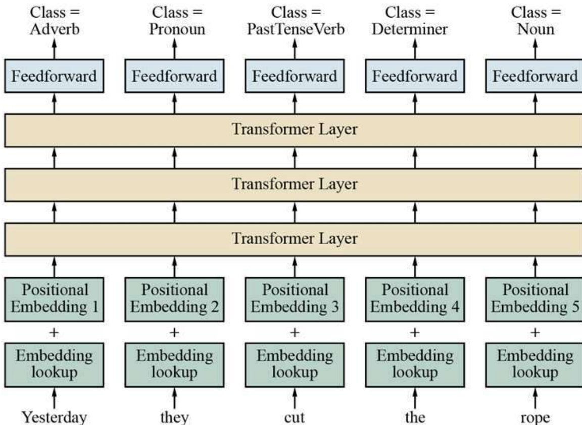
Using the transformer architecture for POS tagging.
