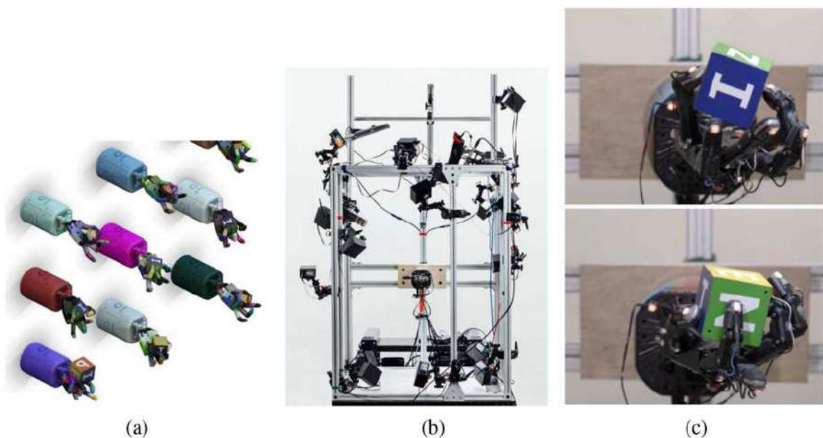
Training a robust policy. (a) Multiple simulations are run of a robot hand manipulating objects, with different randomized parameters for physics and lighting. Courtesy of Wojciech Zaremba. (b) The real-world environment, with a single robot hand in the center of a cage, surrounded by cameras and range
