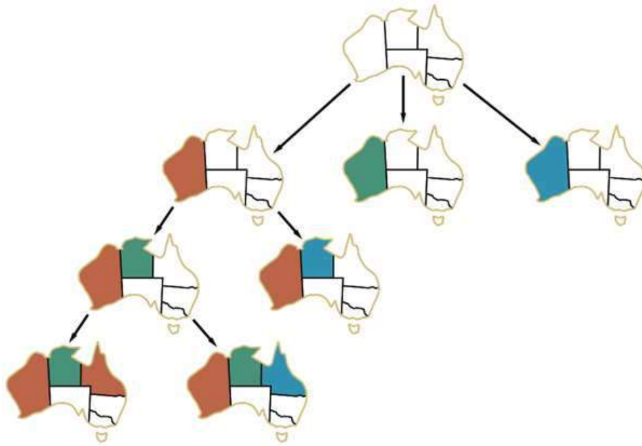
Part of the search tree for the map-coloring problem in Figure 6.1 .
