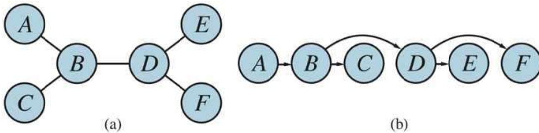
(a) The constraint graph of a tree-structured CSP. (b) A linear ordering of the variables consistent with the tree with A as the root. This is known as a topological sort of the variables.
