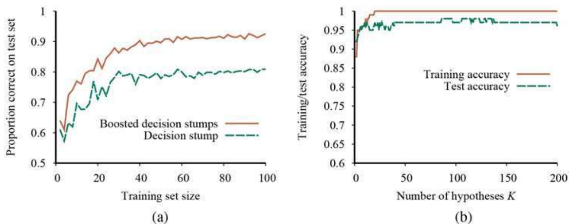
(a) Graph showing the performance of boosted decision stumps with K = 5 versus unboosted decision stumps on the restaurant data. (b) The proportion correct on the training set and the test set as a function of K , the number of hypotheses in the ensemble. Notice that the test set accuracy improves slightly even after the training accuracy reaches 1, i.e., after the ensemble fits the data exactly.
