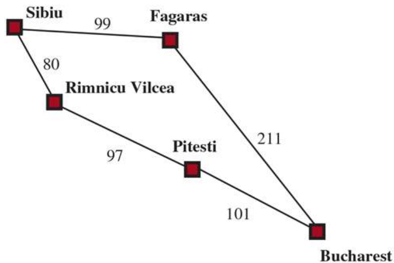
Part of the Romania state space, selected to illustrate uniform-cost search.
