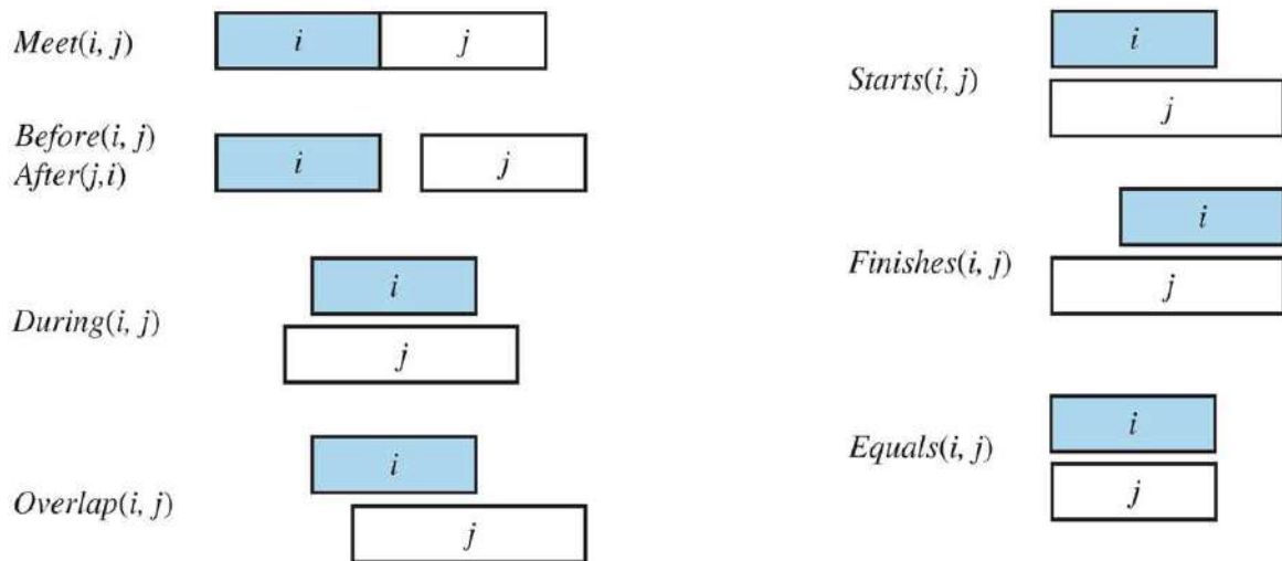
Predicates on time intervals.
