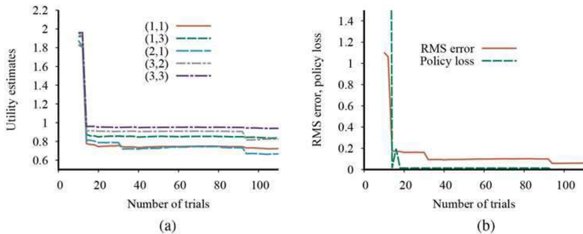
Performance of the exploratory ADP agent using R^+ = 2 and N_e = 5 . (a) Utility estimates for selected states over time. (b) The RMS error in utility values and the associated policy loss.
