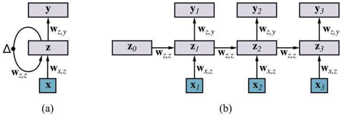
(a) Schematic diagram of an RNN where the hidden layer z has recurrent connections; the \Delta symbol indicates a delay. Each input x is the word embedding vector of the next word in the sentence. Each output y is the output for that time step. (b) The same network unrolled over three timesteps to create a feedforward network. Note that the weights are shared across all timesteps.
