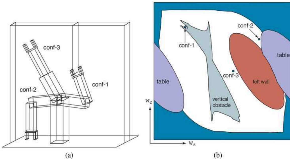
Three robot configurations, shown in workspace and configuration space.
