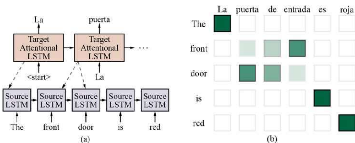
(a) Attentional sequence-to-sequence model for English-to-Spanish translation. The dashed lines represent attention. (b) Example of attention probability matrix for a bilingual sentence pair, with darker boxes representing higher values of a_{ij} . The attention probabilities sum to one over each column.
