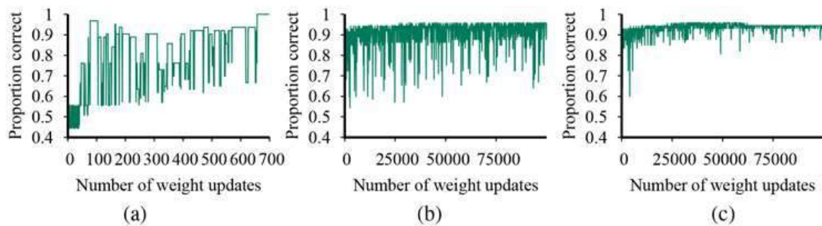
(a) Plot of total training-set accuracy vs. number of iterations through the training set for the perceptron learning rule, given the earthquake/explosion data in Figure 19.15(a) . (b) The same plot for the noisy, nonseparable data in Figure 19.15(b) ; note the change in scale of the x -axis. (c) The same plot as in (b), with a learning rate schedule \alpha(t) = 1000/(1000 + t) .
