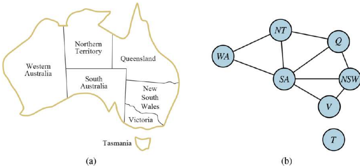
(a) The principal states and territories of Australia. Coloring this map can be viewed as a constraint satisfaction problem (CSP). The goal is to assign colors to each region so that no neighboring regions have the same color. (b) The map-coloring problem represented as a constraint graph.
