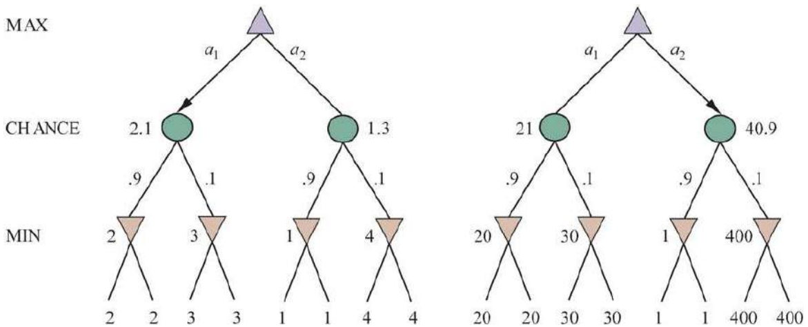
An order-preserving transformation on leaf values changes the best move.
