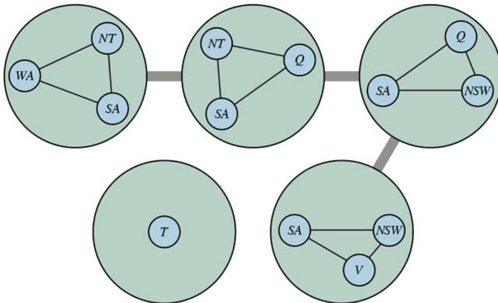
A tree decomposition of the constraint graph in Figure 6.12(a) \square .
