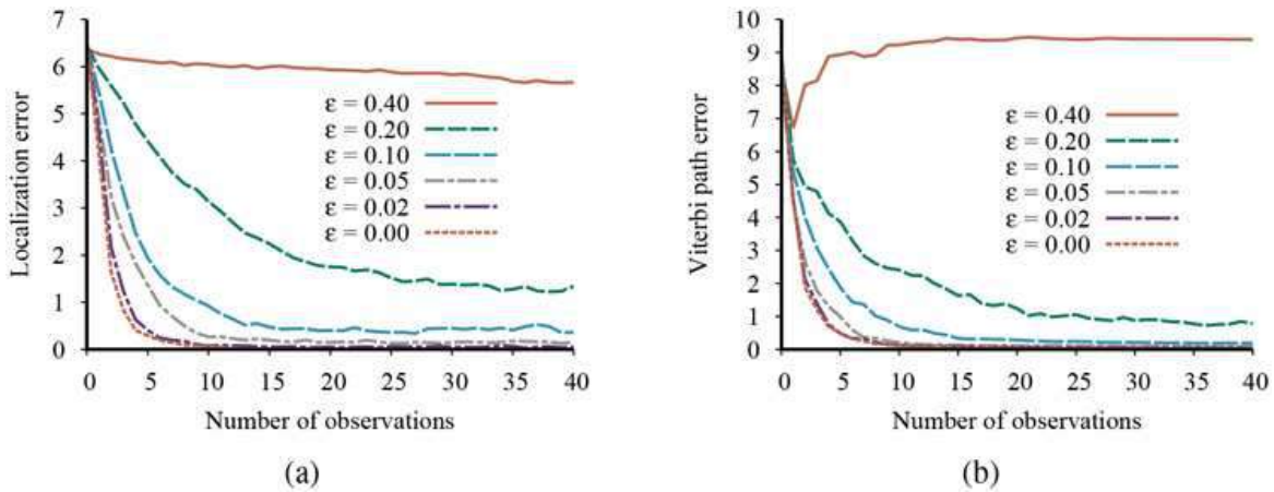
Performance of HMM localization as a function of the length of the observation sequence for various different values of the sensor error probability \epsilon ; data averaged over 400 runs. (a) The localization error, defined as the Manhattan distance from the true location. (b) The Viterbi path error, defined as the average Manhattan distance of states on the Viterbi path from corresponding states on the true path.
