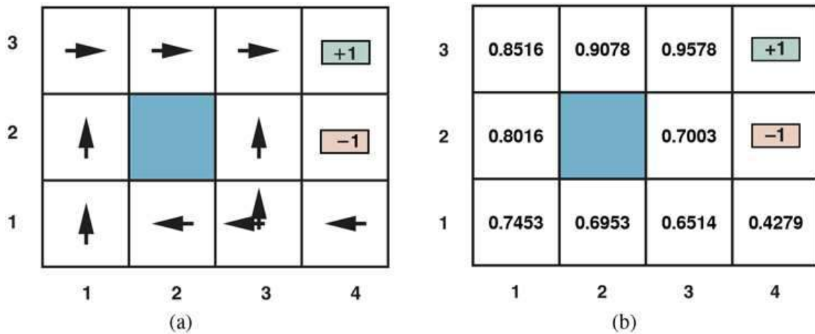
(a) The optimal policies for the stochastic environment with R(s,a,s') = -0.04 for transitions between nonterminal states. There are two policies because in state (3,1) both Left and Up are optimal. We saw this before in Figure 17.2 . (b) The utilities of the states in the 4 \times 3 world, given policy \pi .
