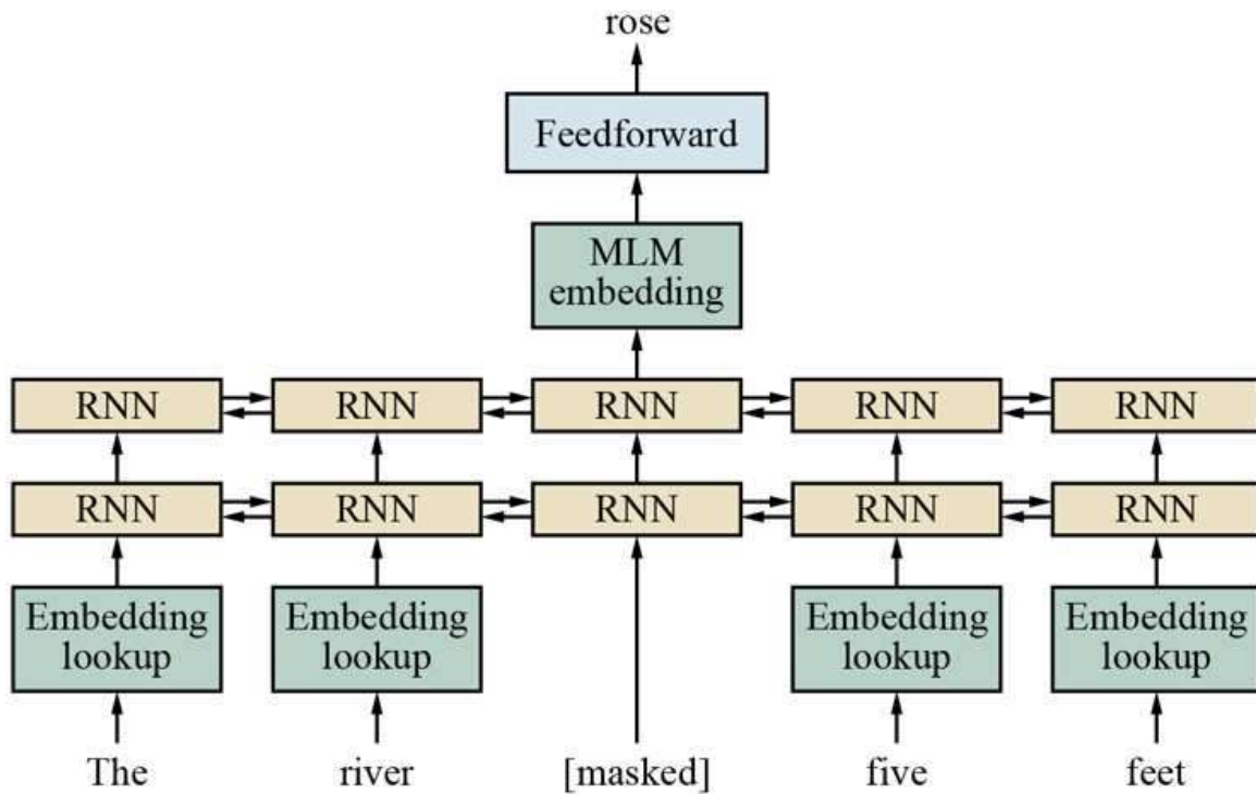
Masked language modeling: pretrain a bidirectional model—for example, a multilayer RNN—by masking input words and predicting only those masked words.
