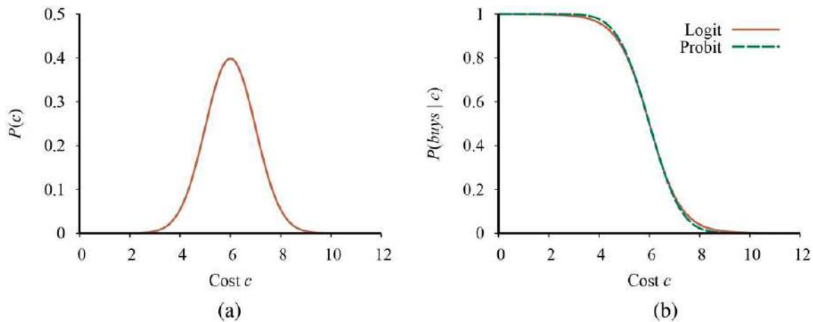
(a) A normal (Gaussian) distribution for the cost threshold, centered on \mu = 6.0 with standard deviation \sigma = 1.0 . (b) Expit and probit models for the probability of buys given cost , for the parameters \mu = 6.0 and \sigma = 1.0 .
