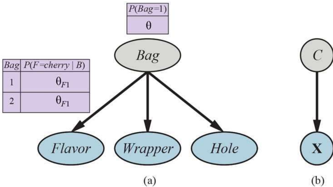
(a) A mixture model for candy. The proportions of different flavors, wrappers, and presence of holes depend on the bag, which is not observed. (b) Bayesian network for a Gaussian mixture. The mean and covariance of the observable variables X depend on the component C .
