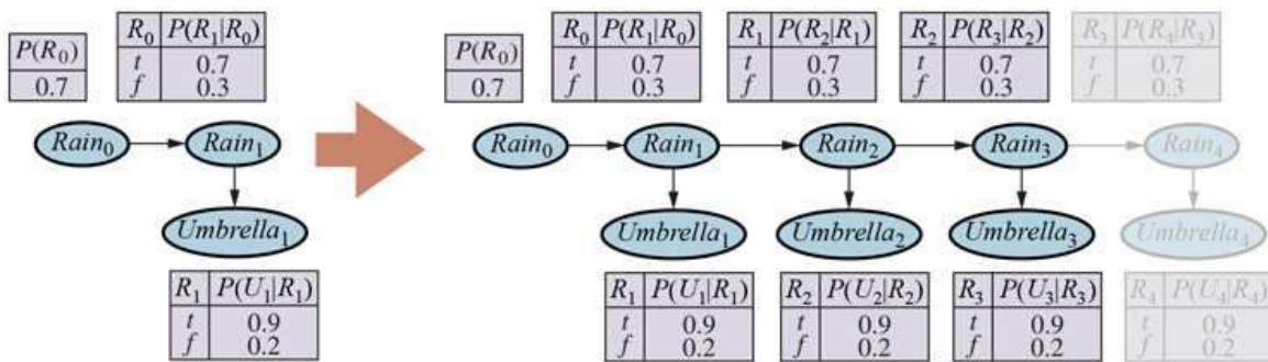
An unrolled dynamic Bayesian network that represents a hidden Markov model (repeat of Figure 14.16 ).
