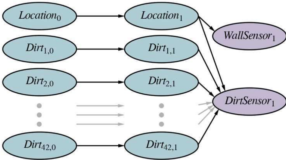
A dynamic Bayes net for simultaneous localization and mapping in the stochastic-dirt vacuum world. Dirty squares persist with probability p , and clean squares become dirty with probability 1 - p . The local dirt sensor is 90% accurate, for the square in which the robot is currently located.
