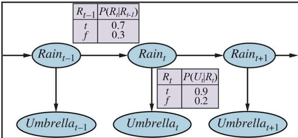
Bayesian network structure and conditional distributions describing the umbrella world. The transition model is \mathbf{P}(Rain_t|Rain_{t-1}) and the sensor model is \mathbf{P}(Umbrella_t|Rain_t) .
