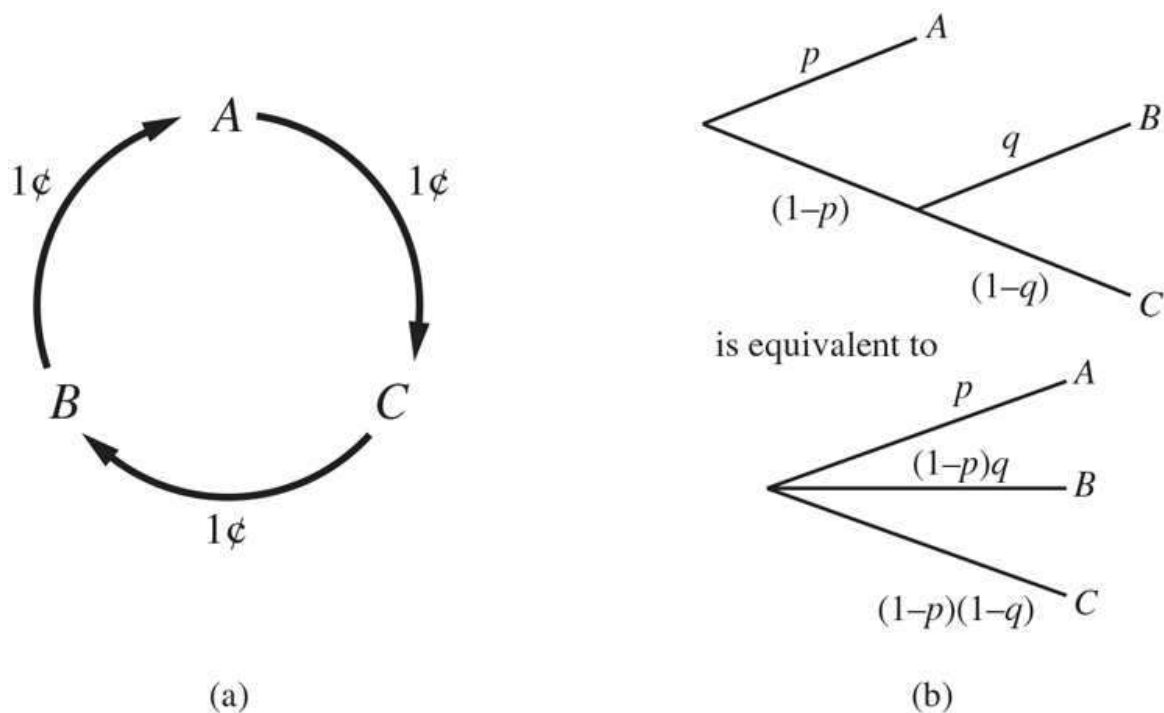
(a) Nontransitive preferences A \succ B \succ C \succ A can result in irrational behavior: a cycle of exchanges each costing one cent. (b) The decomposability axiom.
