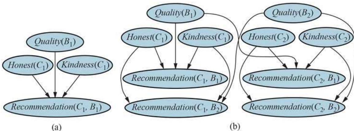
(a) Bayes net for a single customer C_1 recommending a single book B_1 . Honest(C_1) is Boolean, while the other variables have integer values from 1 to 5. (b) Bayes net with two customers and two books.
