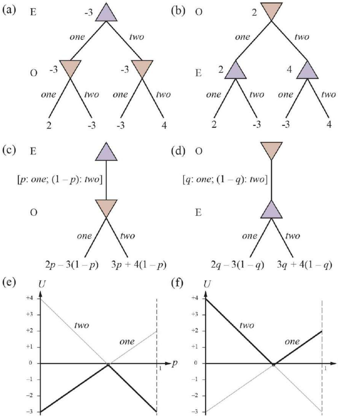
(a) and (b): Minimax game trees for two-finger Morra if the players take turns playing pure strategies. (c) and (d): Parameterized game trees where the first player plays a mixed strategy. The payoffs depend on the probability parameter ( p or q ) in the mixed strategy. (e) and (f): For any particular value of the probability parameter, the second player will choose the "better" of the two actions, so the value of the first player's mixed strategy is given by the heavy lines. The first player will choose the probability parameter for the mixed strategy at the intersection point.
