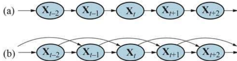
(a) Bayesian network structure corresponding to a first-order Markov process with state defined by the variables \mathbf{X}_t . (b) A second-order Markov process.
