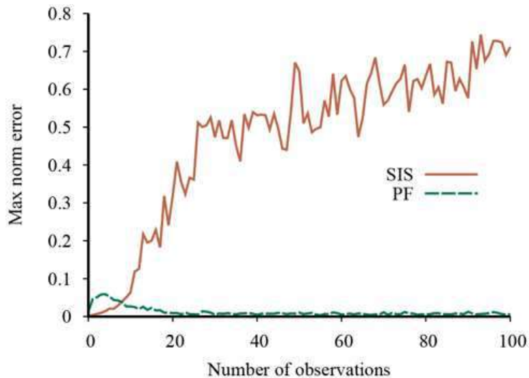
Max norm error in the grid-world location estimate (compared to exact inference) for likelihood weighting (sequential importance sampling) with 100,000 samples and particle filtering with 1,000 samples; data averaged over 50 runs.
