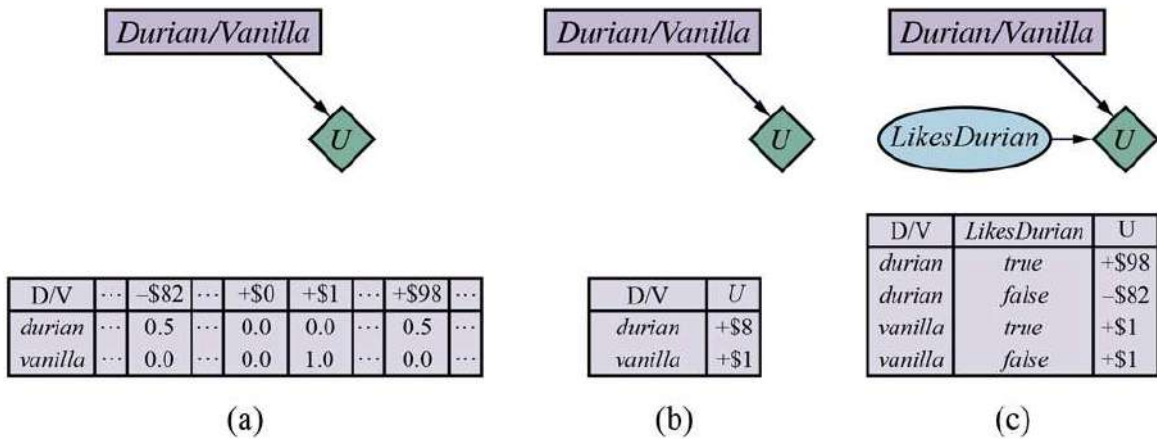
(a) A decision network for the ice cream choice with an uncertain utility function. (b) The network with the expected utility of each action. (c) Moving the uncertainty from the utility function into a new random variable.
