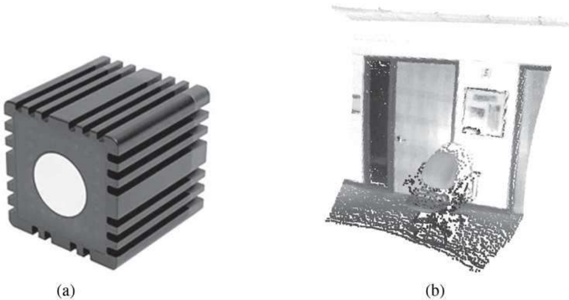
(a) Time-of-flight camera; image courtesy of Mesa Imaging GmbH. (b) 3D range image obtained with this camera. The range image makes it possible to detect obstacles and objects in a robot's vicinity. Image courtesy of Willow Garage, LLC.
