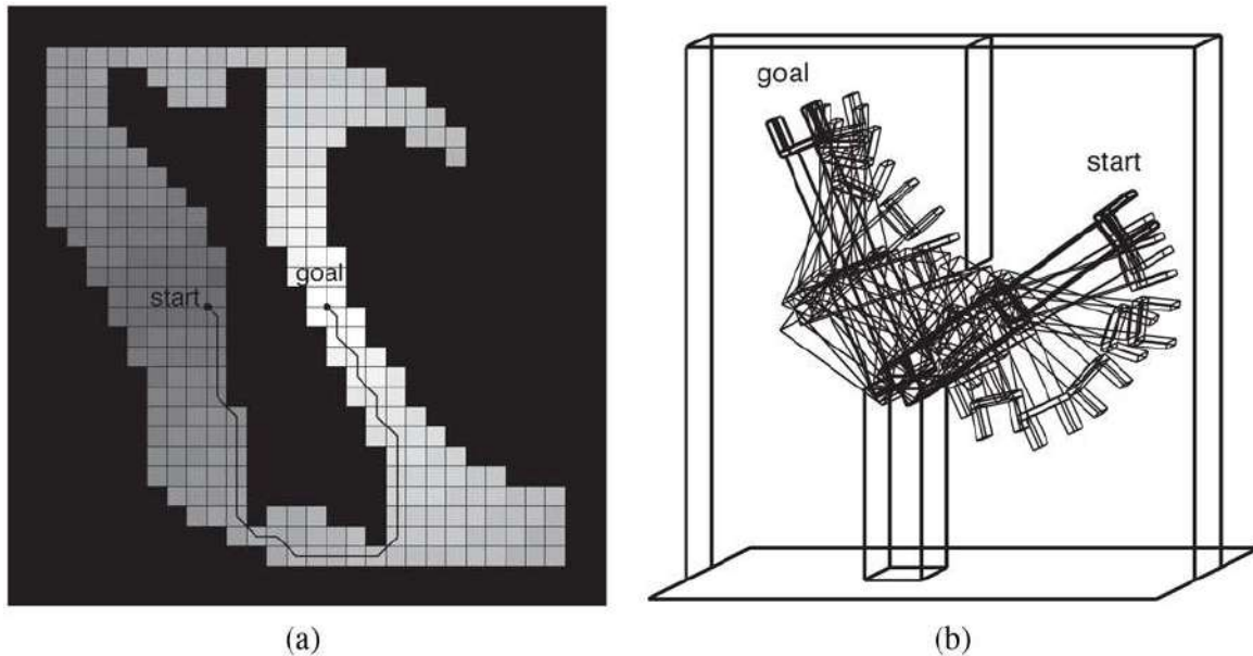
(a) Value function and path found for a discrete grid cell approximation of the configuration space. (b) The same path visualized in workspace coordinates. Notice how the robot bends its elbow to avoid a collision with the vertical obstacle.
