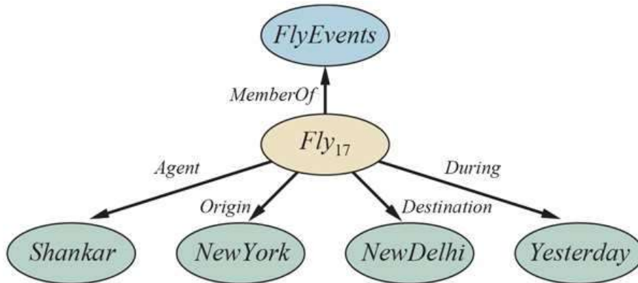
A fragment of a semantic network showing the representation of the logical assertion Fly(Shankar, NewYork, NewDelhi, Yesterday) .
