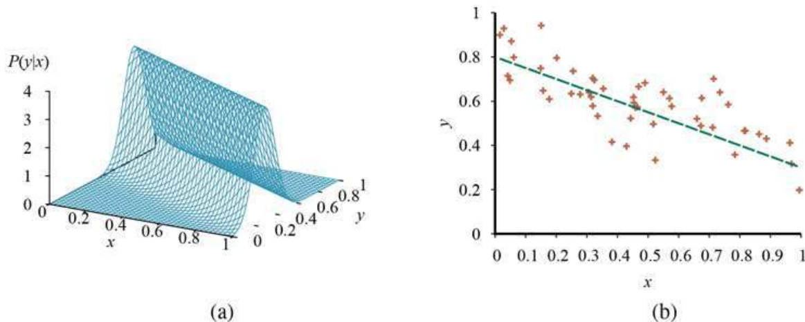
(a) A linear–Gaussian model described as y = \theta_1 x + \theta_2 plus Gaussian noise with fixed variance. (b) A set of 50 data points generated from this model and the best-fit line.
