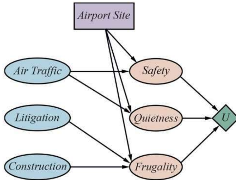
A decision network for the airport-siting problem.
