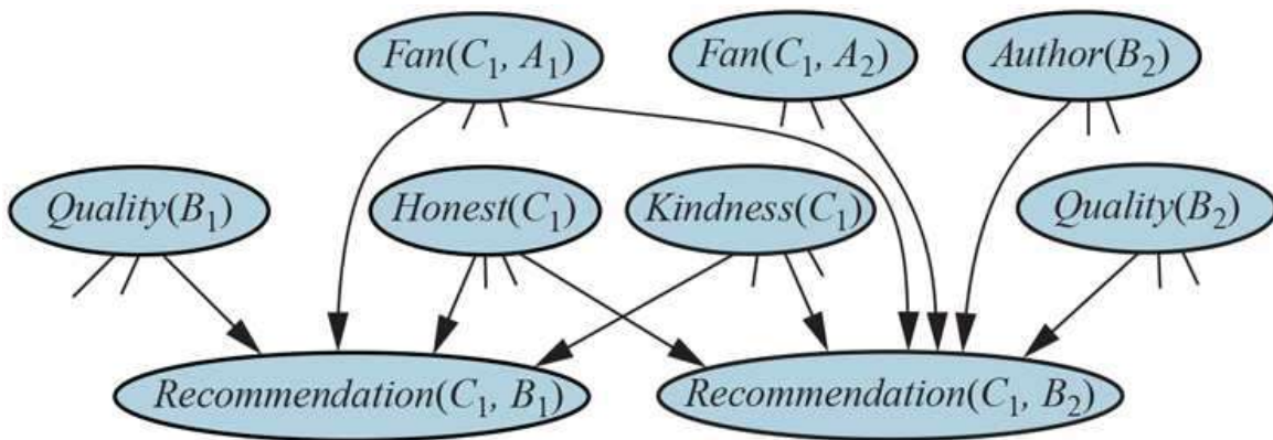
Fragment of the equivalent Bayes net for the book recommendation RPM when Author(B_2) is unknown.
