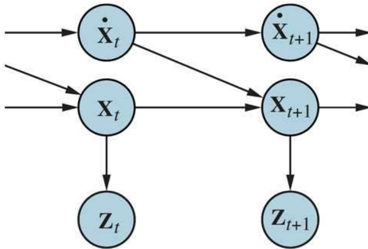
Bayesian network structure for a linear dynamical system with position \mathbf{X}_t , velocity \dot{\mathbf{X}}_t , and position measurement \mathbf{Z}_t .
