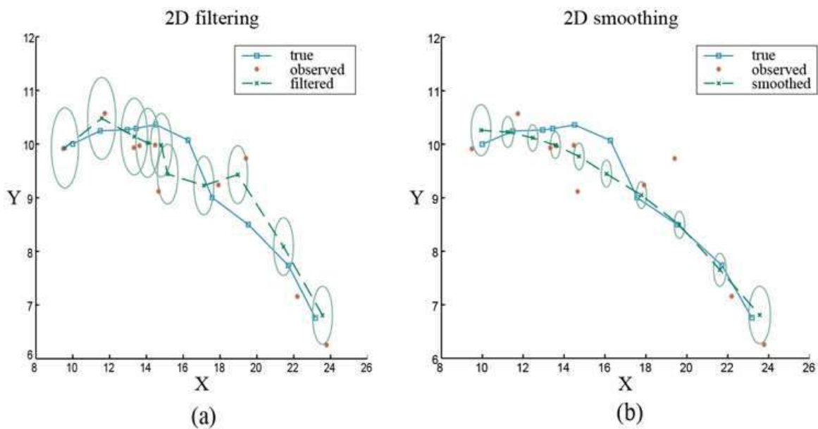
(a) Results of Kalman filtering for an object moving on the X - Y plane, showing the true trajectory (left to right), a series of noisy observations, and the trajectory estimated by Kalman filtering. Variance in the position estimate is indicated by the ovals. (b) The results of Kalman smoothing for the same observation sequence.
