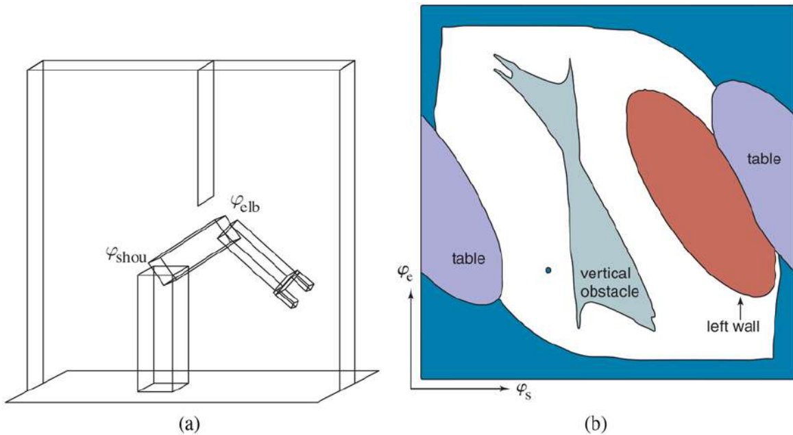
(a) Workspace representation of a robot arm with two degrees of freedom. The workspace is a box with a flat obstacle hanging from the ceiling. (b) Configuration space of the same robot. Only white regions in the space are configurations that are free of collisions. The dot in this diagram corresponds to the configuration of the robot shown on the left.
