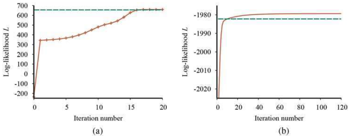
Graphs showing the log likelihood of the data, L , as a function of the EM iteration. The horizontal line shows the log likelihood according to the true model. (a) Graph for the Gaussian mixture model in Figure 20.12 . (b) Graph for the Bayesian network in Figure 20.14(a) .
