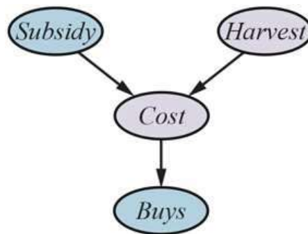
A simple network with discrete variables ( Subsidy and Buys ) and continuous variables ( Harvest and Cost ).
