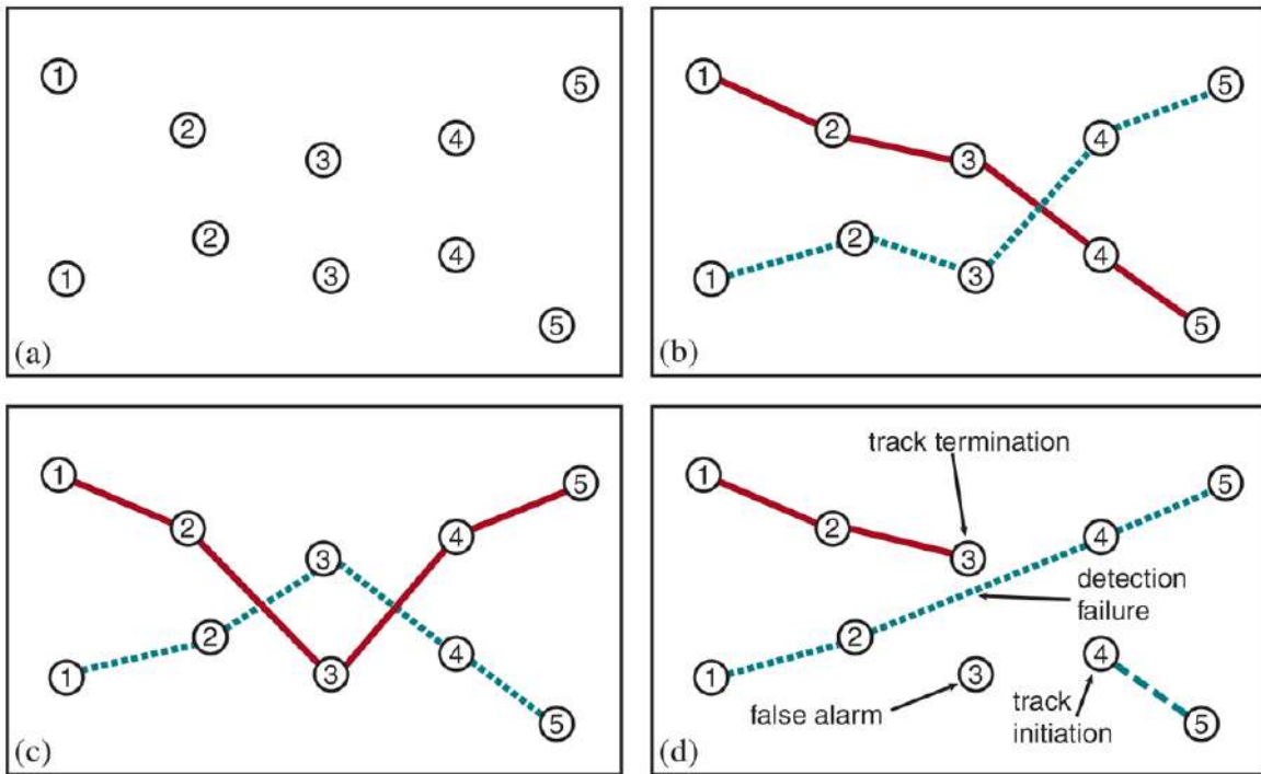
(a) Observations made of object locations in 2D space over five time steps. Each observation blip is labeled with the time step but does not identify the object that produced it. (b–c) Possible hypotheses about the underlying object tracks. (d) A hypothesis for the case in which false alarms, detection failures, and track initiation/termination are possible.
