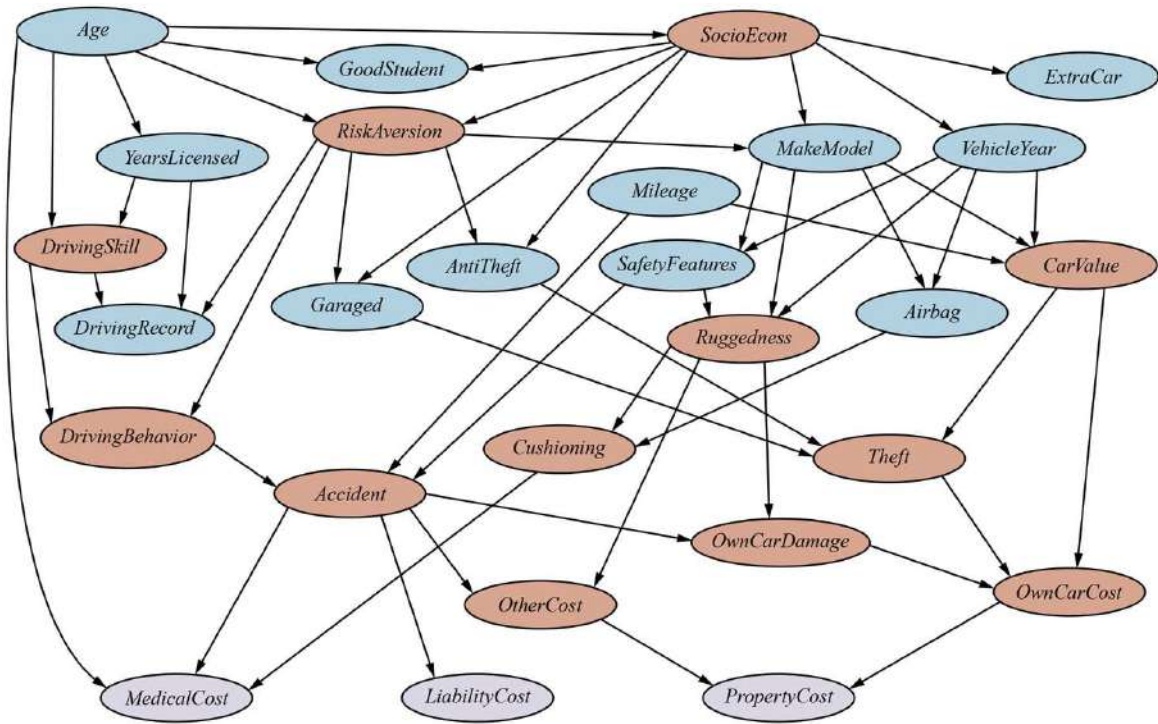
A Bayesian network for evaluating car insurance applications.
