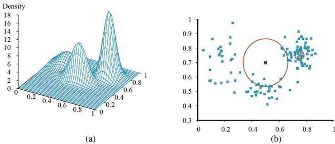
(a) A 3D plot of the mixture of Gaussians from Figure 20.12(a) . (b) A 128-point sample of points from the mixture, together with two query points (small orange squares) and their 10-nearest-neighborhoods (large circle and smaller circle to the right).
