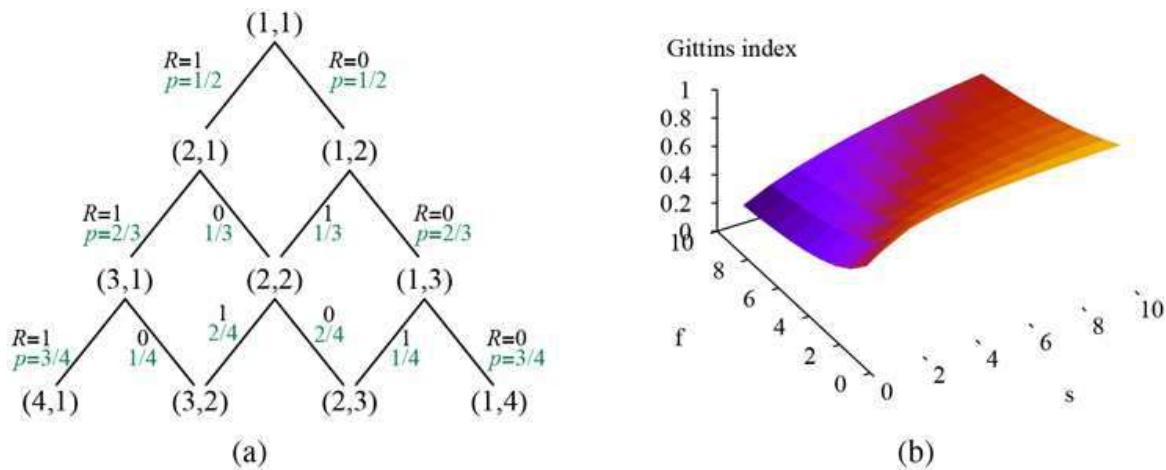
(a) States, rewards, and transition probabilities for the Bernoulli bandit. (b) Gittins indices for the states of the Bernoulli bandit process.
