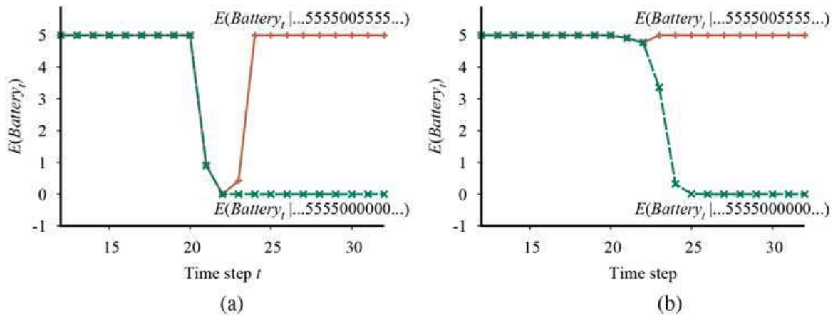
(a) Upper curve: trajectory of the expected value of Battery_t for an observation sequence consisting of all 5s except for 0s at t = 21 and t = 22 , using a simple Gaussian error model. Lower curve: trajectory when the observation remains at 0 from t = 21 onwards. (b) The same experiment run with the transient failure model. The transient failure is handled well, but the persistent failure results in excessive pessimism about the battery charge.
