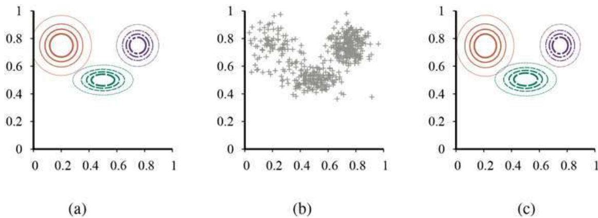
(a) A Gaussian mixture model with three components; the weights (left-to-right) are 0.2, 0.3, and 0.5. (b) 500 data points sampled from the model in (a). (c) The model reconstructed by EM from the data in (b).
