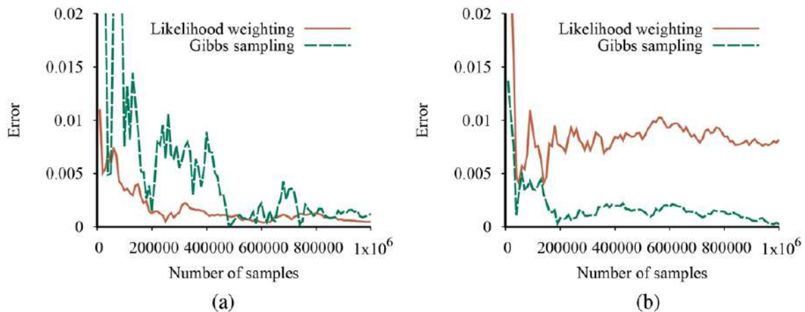
Performance of Gibbs sampling compared to likelihood weighting on the car insurance network: (a) for the standard query on PropertyCost , and (b) for the case where the output variables are observed and Age is the query variable.
