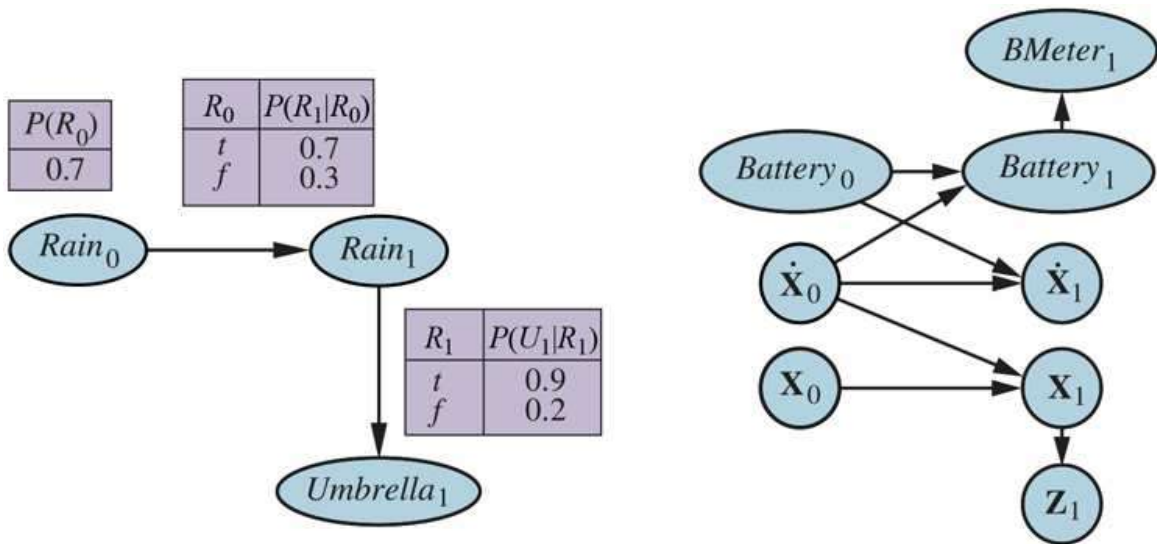
Left: Specification of the prior, transition model, and sensor model for the umbrella DBN. Subsequent slices are copies of slice 1. Right: A simple DBN for robot motion in the X–Y plane.
