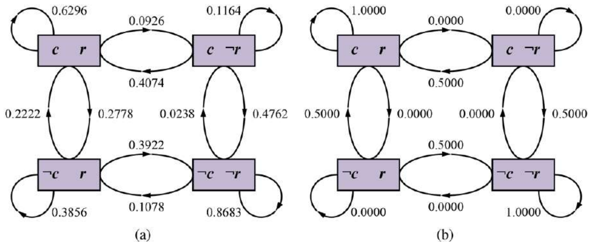
(a) The states and transition probabilities of the Markov chain for the query \mathbf{P}(\text{Rain}|\text{Sprinkler} = \text{true}, \text{WetGrass} = \text{true}) . Note the self-loops: the state stays the same when either variable is chosen and then resamples the same value it already has. (b) The transition probabilities when the CPT for Rain constrains it to have the same value as Cloudy .
