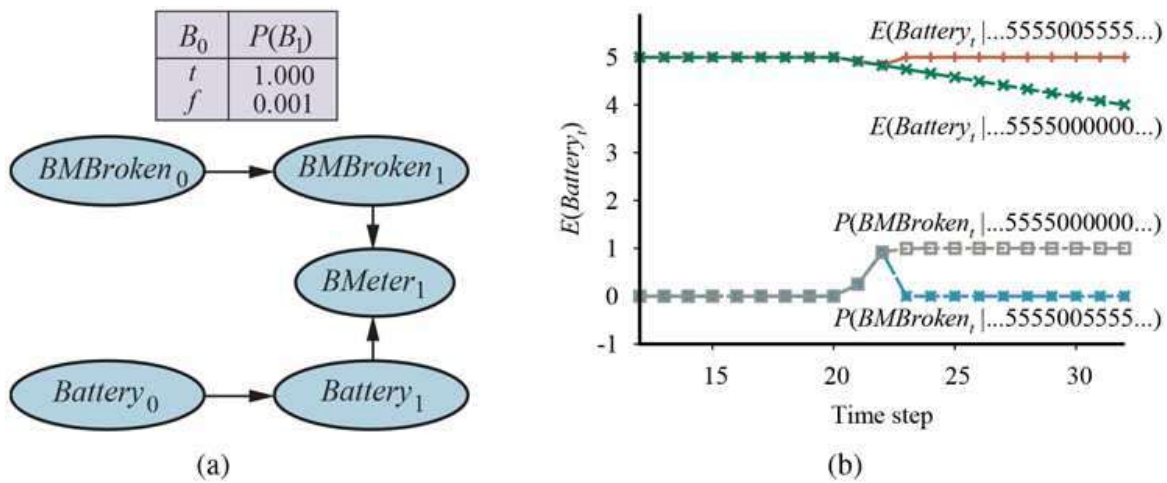
(a) A DBN fragment showing the sensor status variable required for modeling persistent failure of the battery sensor. (b) Upper curves: trajectories of the expected value of Battery_t for the “transient failure” and “permanent failure” observations sequences. Lower curves: probability trajectories for BMBroken given the two observation sequences.
