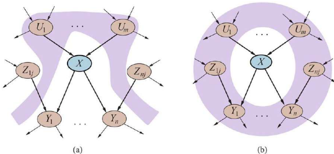
(a) A node X is conditionally independent of its non-descendants (e.g., the Z_{ij} s) given its parents (the U_i s shown in the gray area). (b) A node X is conditionally independent of all other nodes in the network given its Markov blanket (the gray area).
