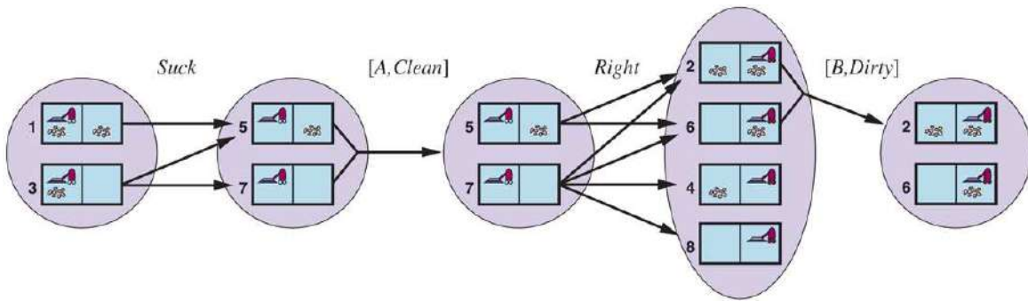
Two prediction–update cycles of belief-state maintenance in the kindergarten vacuum world with local sensing.
