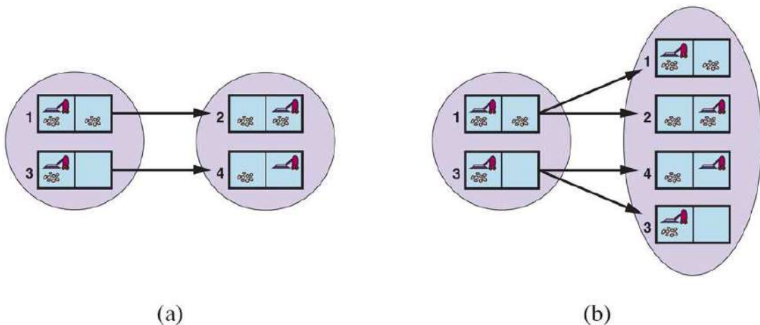
(a) Predicting the next belief state for the sensorless vacuum world with the deterministic action, Right . (b) Prediction for the same belief state and action in the slippery version of the sensorless vacuum world.
