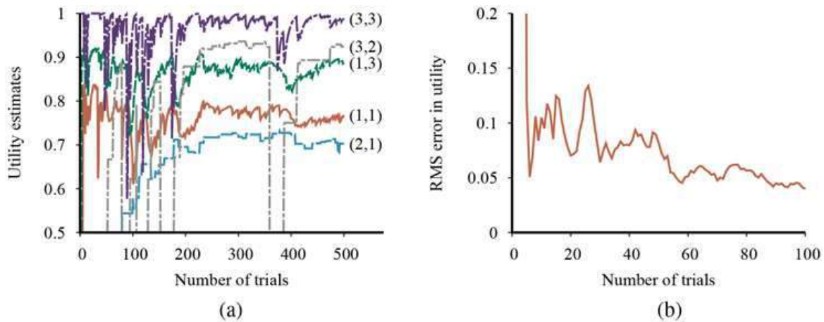
The TD learning curves for the 4 \times 3 world. (a) The utility estimates for a selected subset of states, as a function of the number of trials, for a single run of 500 trials. Compare with the run of 100 trials in Figure 22.3(a) . (b) The root-mean-square error in the estimate for U(1,1) , averaged over 50 runs of 100 trials each.
