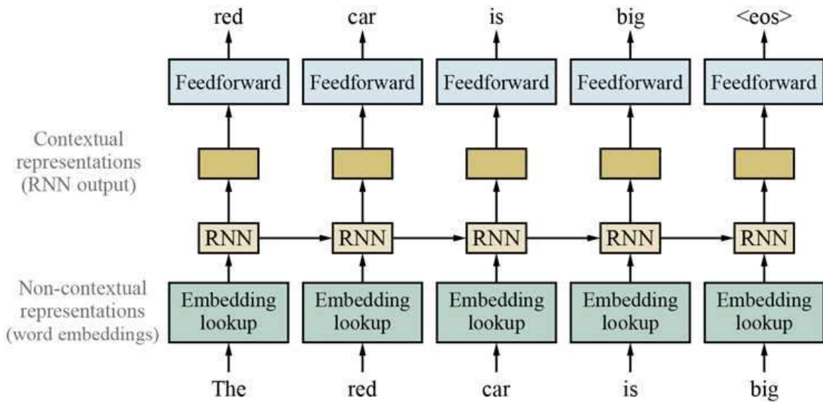
Training contextual representations using a left-to-right language model.
