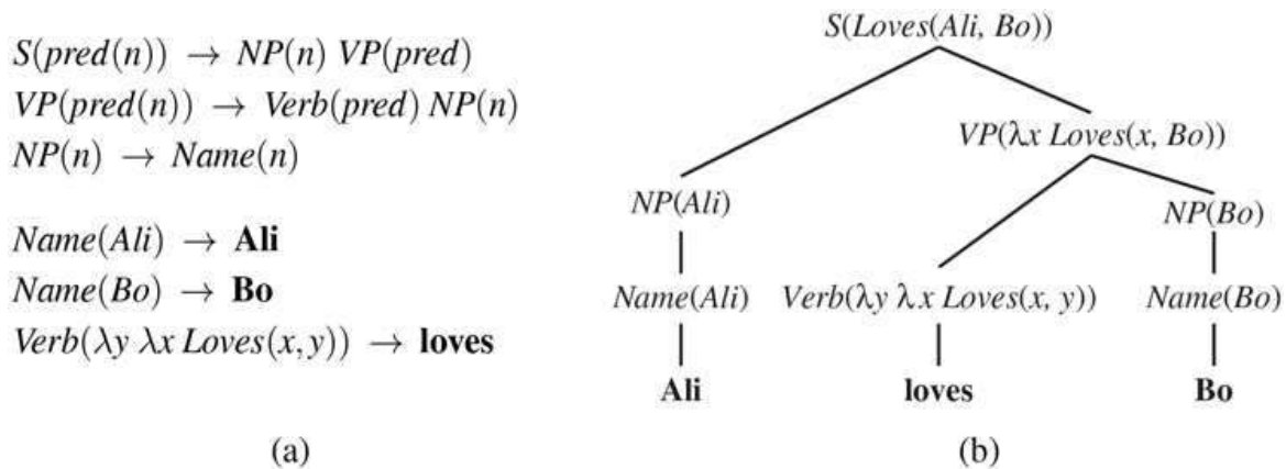
(a) A grammar that can derive a parse tree and semantic interpretation for “Ali loves Bo” (and three other sentences). Each category is augmented with a single argument representing the semantics. (b) A parse tree with semantic interpretations for the string “Ali loves Bo.”
