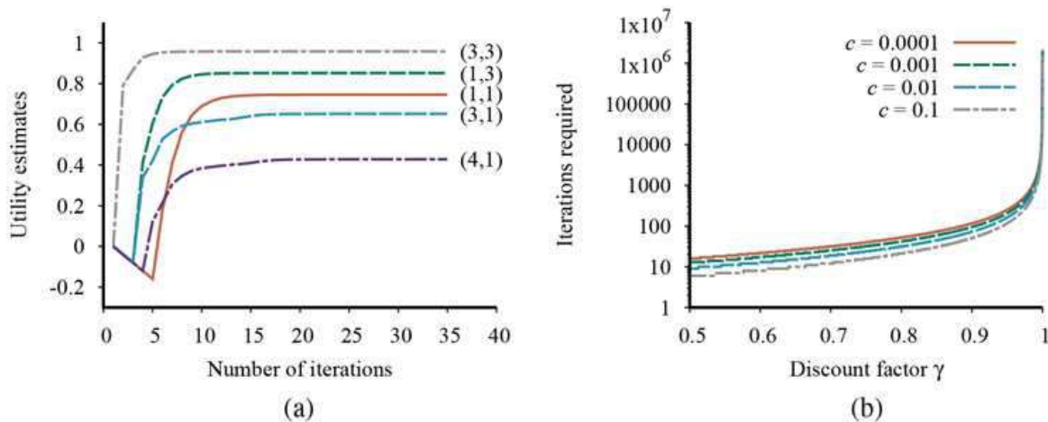
(a) Graph showing the evolution of the utilities of selected states using value iteration. (b) The number of value iterations required to guarantee an error of at most \epsilon = c \cdot R_{\max} , for different values of c , as a function of the discount factor \gamma .
